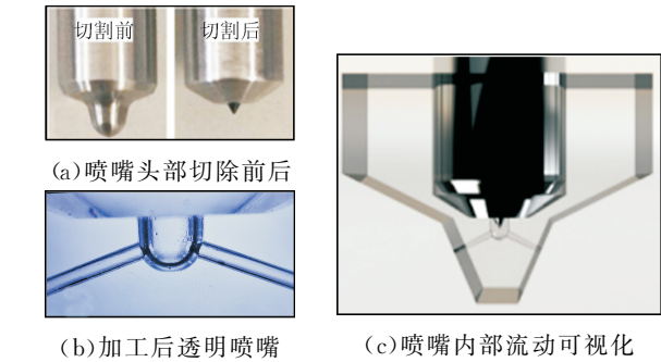
图 2 透明喷嘴头部加工原理及过程 Fig.2 Processing principle and process of theoptical nozzle tip
