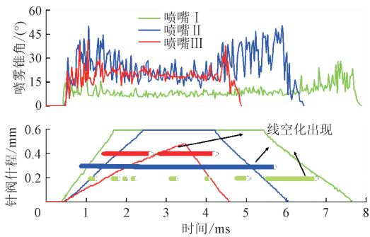
图 8 喷孔直径对喷嘴的针阀升程、线空化及喷雾锥角特性的影响( P_{in}=50 MPa) Fig. 8 Effects of nozzle hole diameter on needle lift, string cavitation and spray ( P_{in}=50 MPa)
