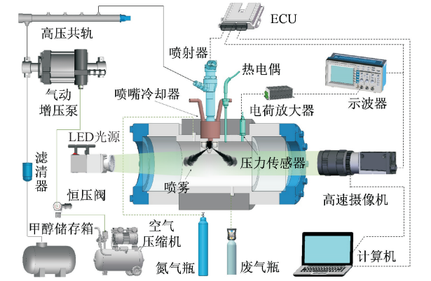
图 1 甲醇高压喷射喷嘴内流及喷雾光学试验台 Fig.1 Optical experimental platform for high-pressure methanol nozzle internal flow and spray
